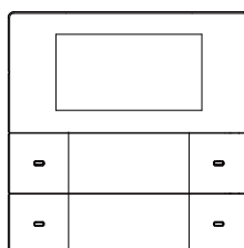
Label models
